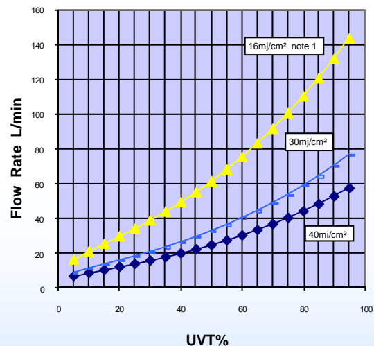
UVD600 Performance Curves note 2
